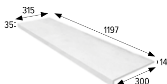
Straight stair-tread 120
