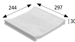
Overflow channel*
