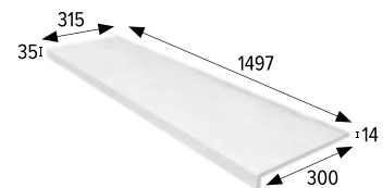
Straight stair-tread 180
