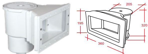
SKLG Model
